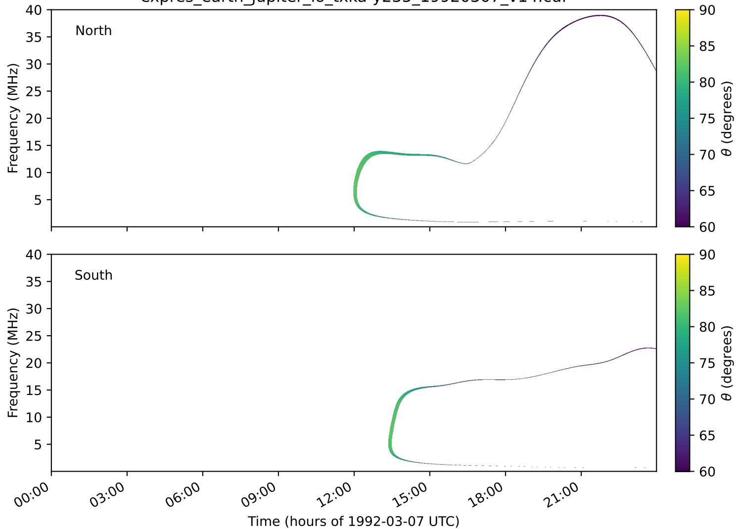
expres_earth_jupiter_io_txka-y235_19920307_v14.cdf
