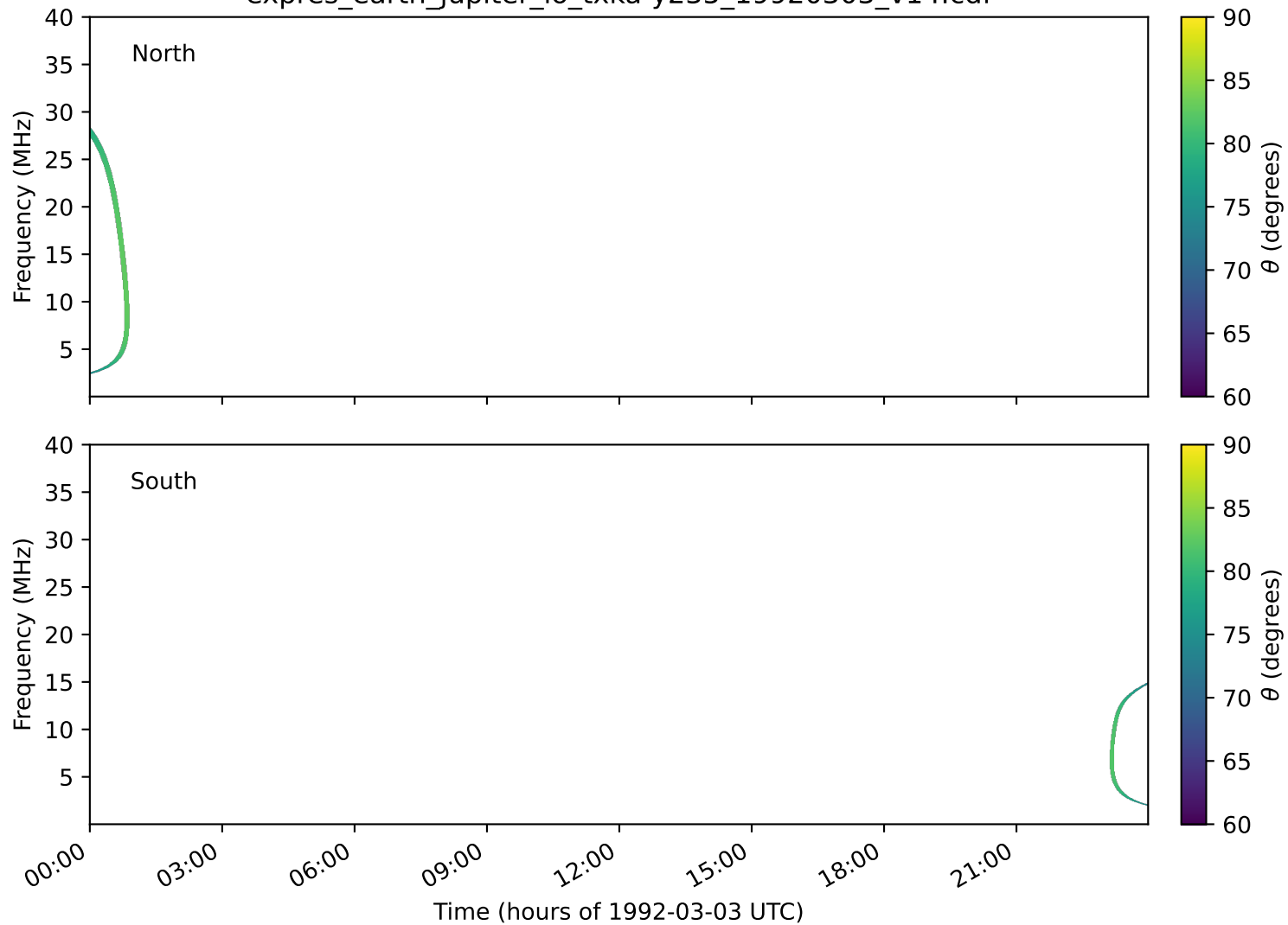
expres_earth_jupiter_io_txka-y235_19920303_v14.cdf
