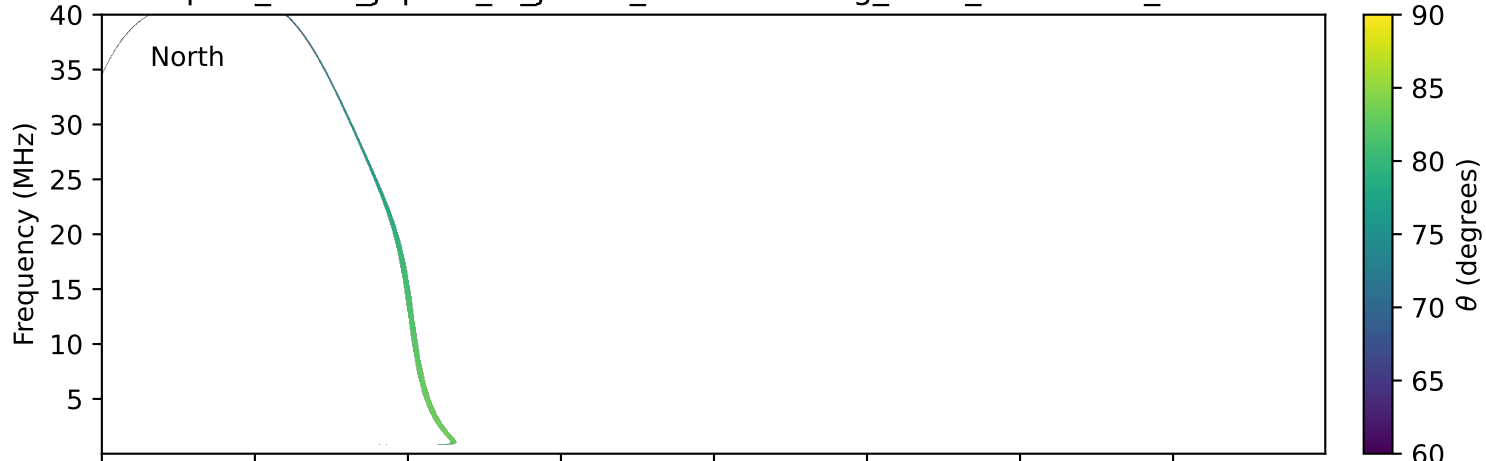
expres_earth_jupiter_io_jrm33_lossc-wid1deg_3kev_19920331_v11.cdf
