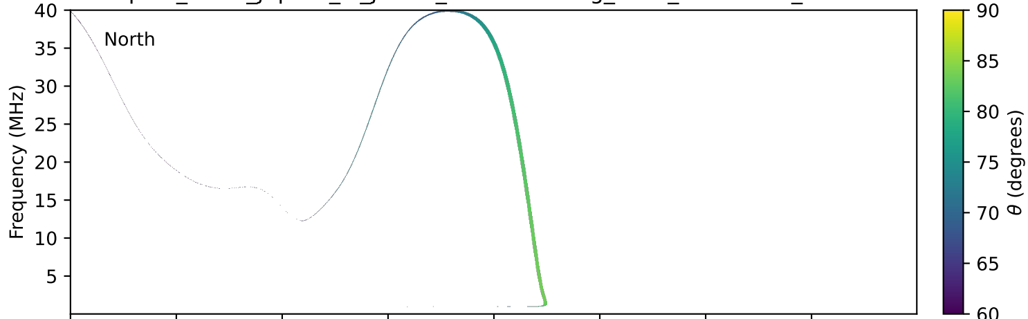
expres_earth_jupiter_io_jrm33_lossc-wid1deg_3kev_19920329_v11.cdf
