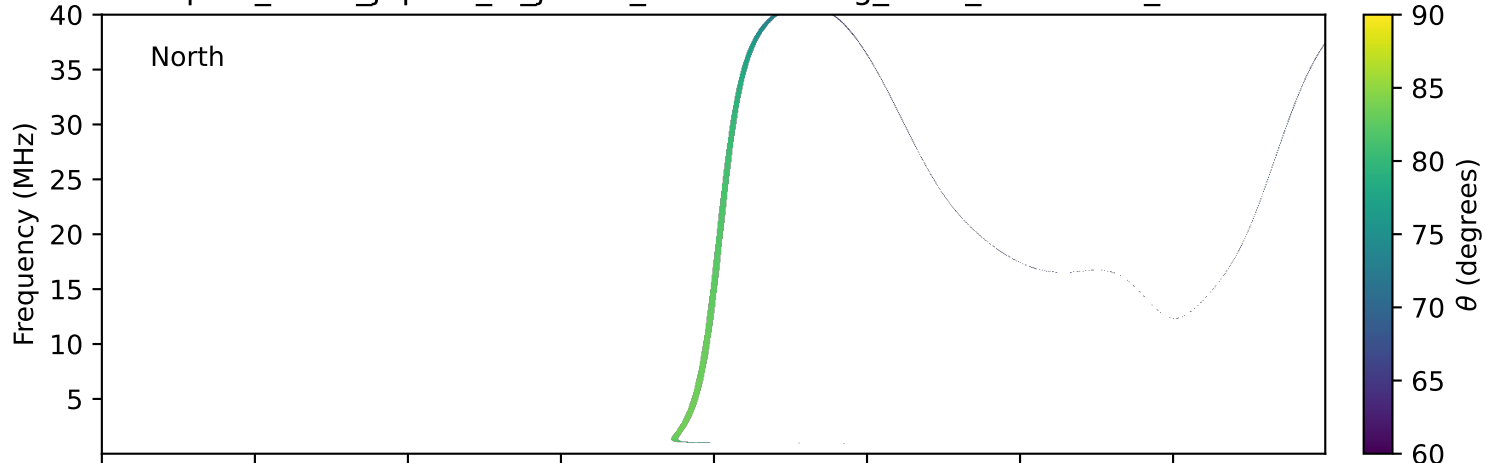
expres_earth_jupiter_io_jrm33_lossc-wid1deg_3kev_19920323_v11.cdf
