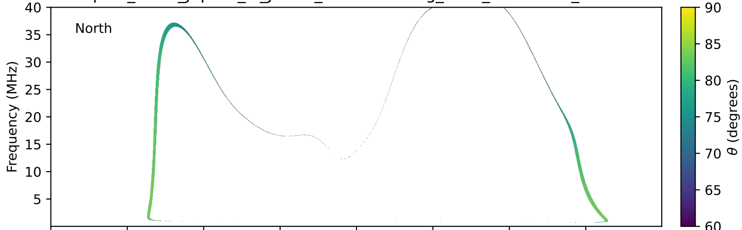
expres_earth_jupiter_io_jrm33_lossc-wid1deg_3kev_19920318_v11.cdf
