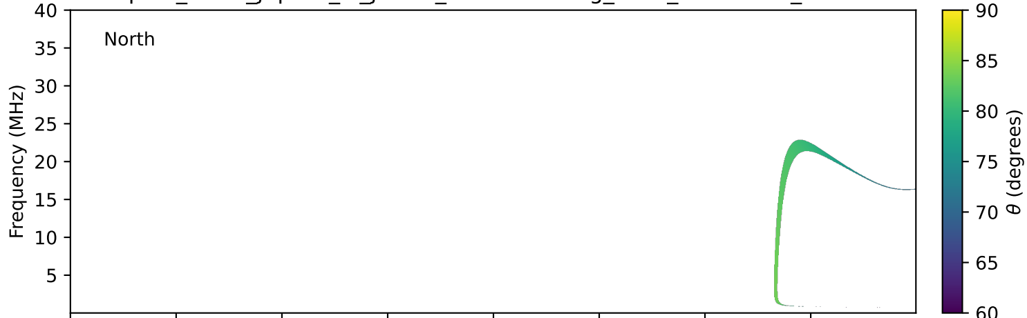
expres_earth_jupiter_io_jrm33_lossc-wid1deg_3kev_19920312_v11.cdf
