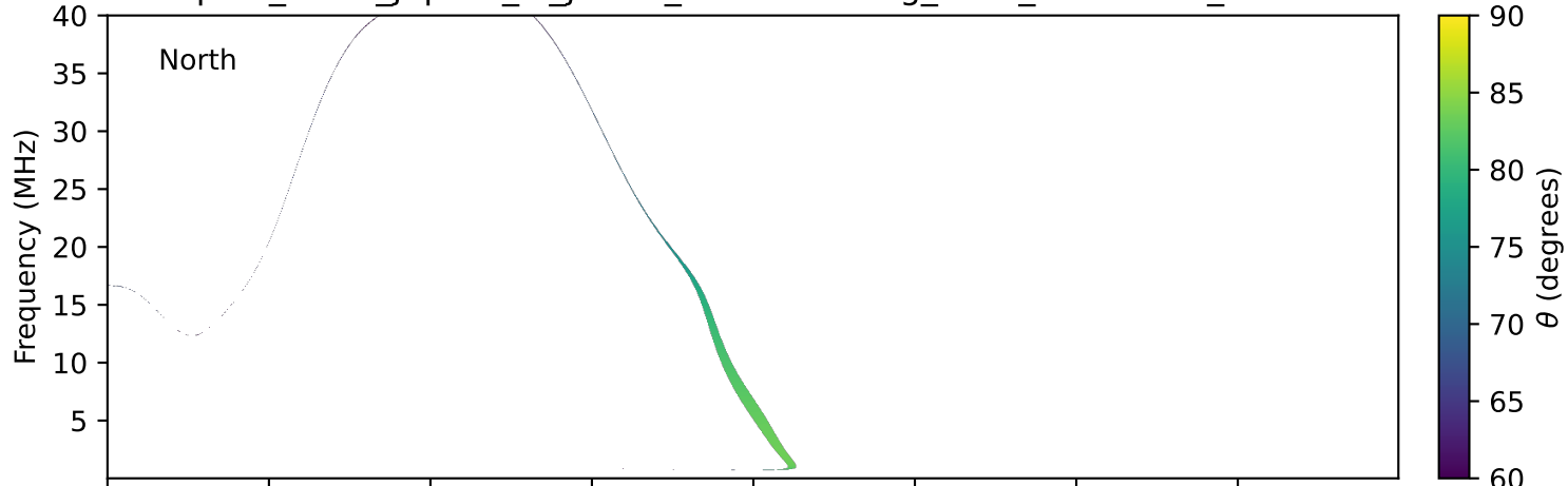
expres_earth_jupiter_io_jrm33_lossc-wid1deg_3kev_19920306_v11.cdf
