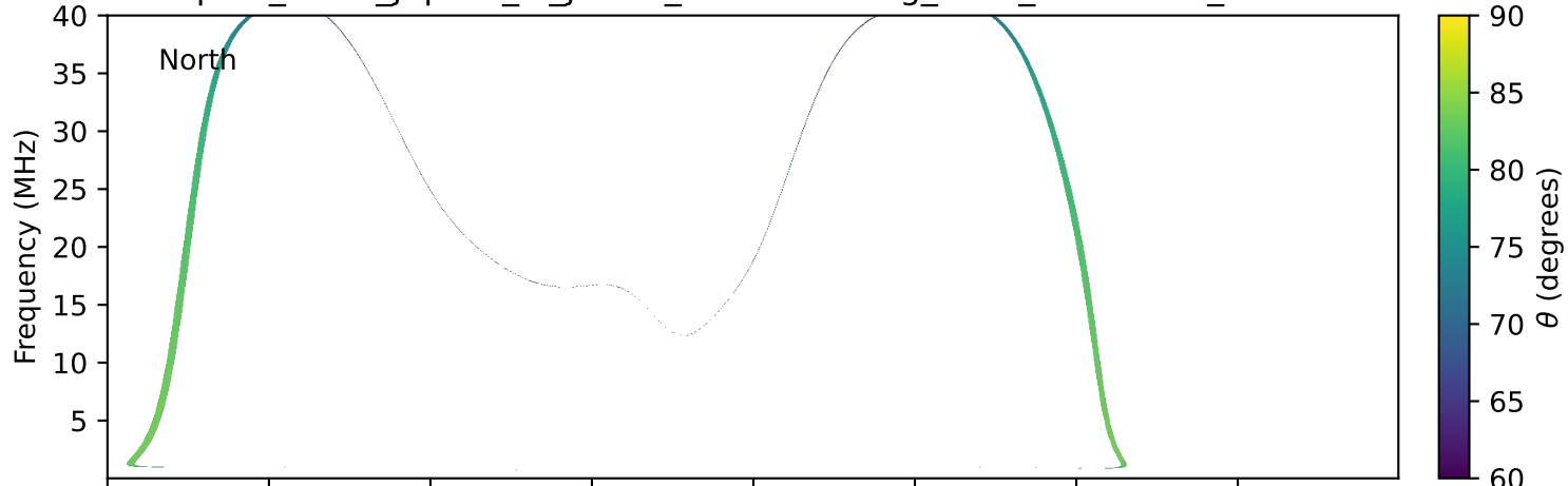
expres_earth_jupiter_io_jrm33_lossc-wid1deg_3kev_19920304_v11.cdf
