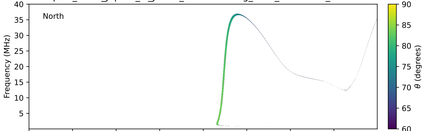
expres_earth_jupiter_io_jrm09_lossc-wid1deg_3kev_19920330_v11.cdf
