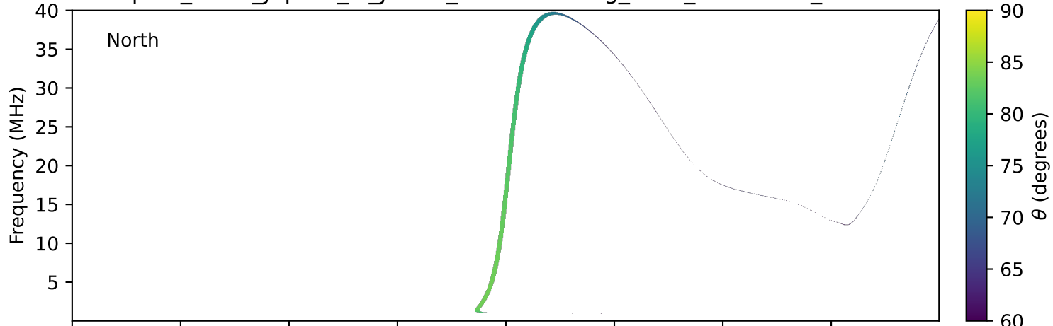
expres_earth_jupiter_io_jrm09_lossc-wid1deg_3kev_19920323_v11.cdf
