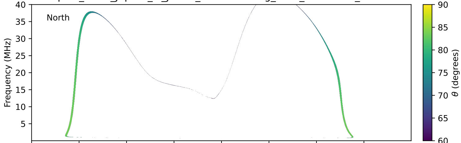
expres_earth_jupiter_io_jrm09_lossc-wid1deg_3kev_19920311_v11.cdf
