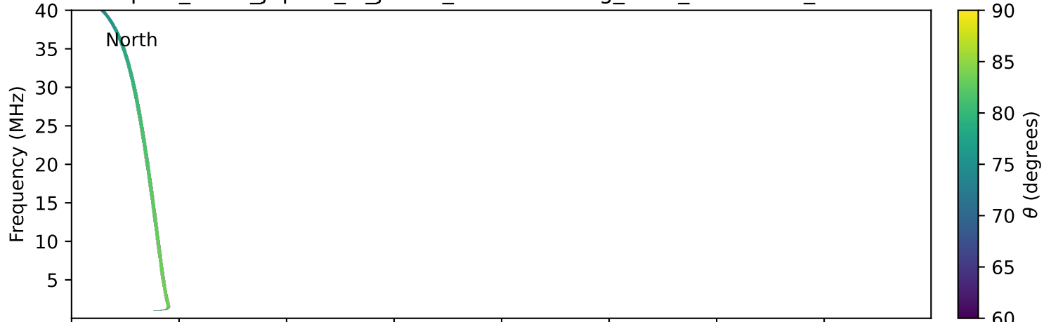
expres_earth_jupiter_io_jrm09_lossc-wid1deg_3kev_19920310_v11.cdf
