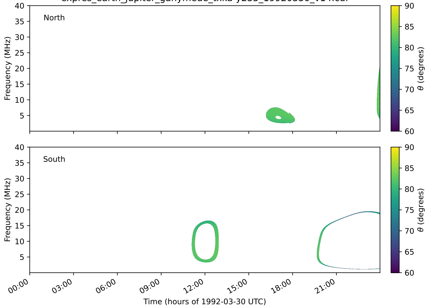
expres_earth_jupiter_ganymede_txka-y235_19920330_v14.cdf
