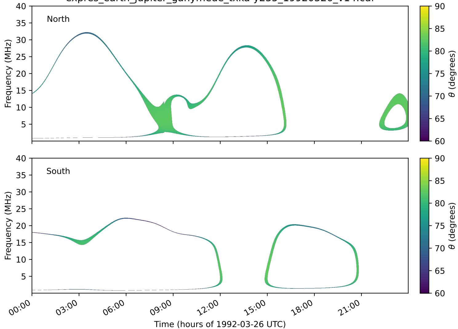
expres_earth_jupiter_ganymede_txka-y235_19920326_v14.cdf
