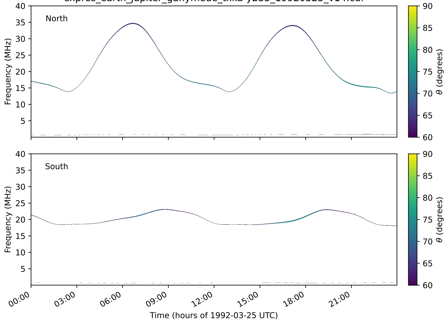
expres_earth_jupiter_ganymede_txka-y235_19920325_v14.cdf
