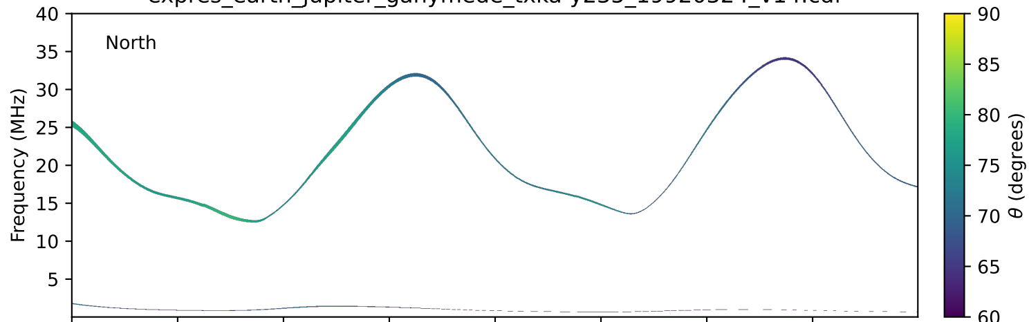
expres_earth_jupiter_ganymede_txka-y235_19920324_v14.cdf
