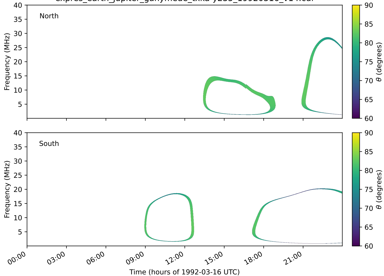
expres_earth_jupiter_ganymede_txka-y235_19920316_v14.cdf
