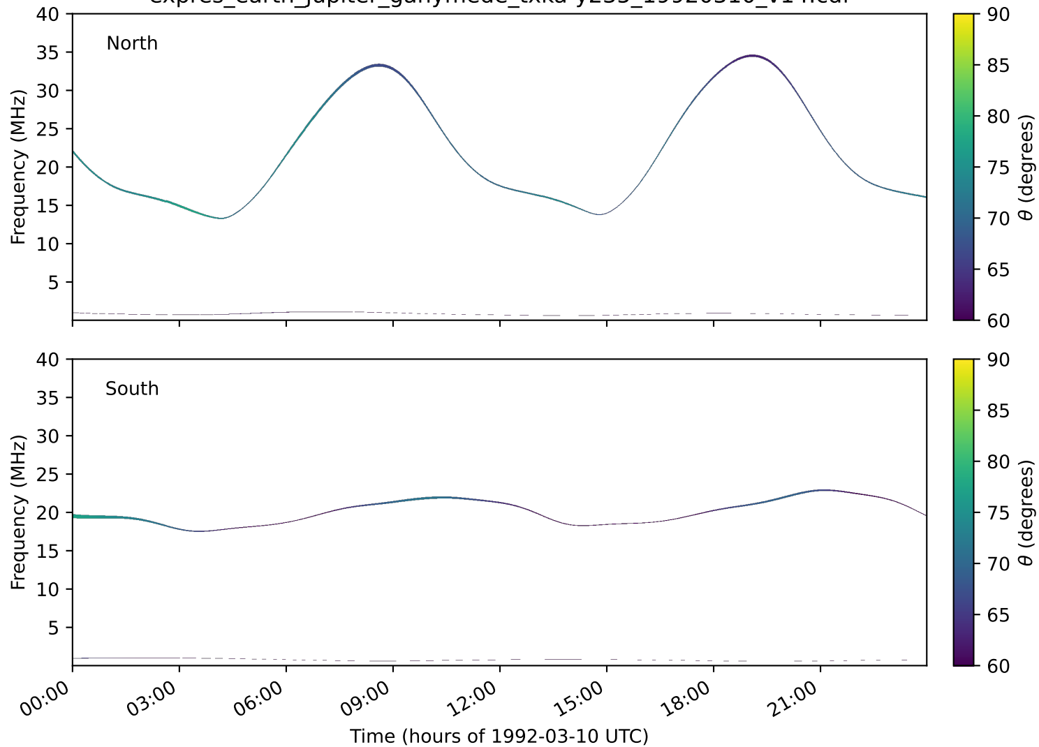
expres_earth_jupiter_ganymede_txka-y235_19920310_v14.cdf
