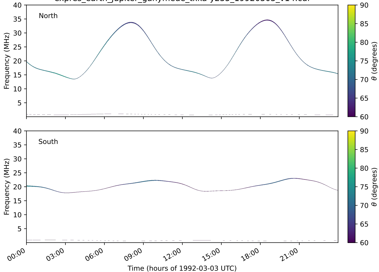
expres_earth_jupiter_ganymede_txka-y235_19920303_v14.cdf
