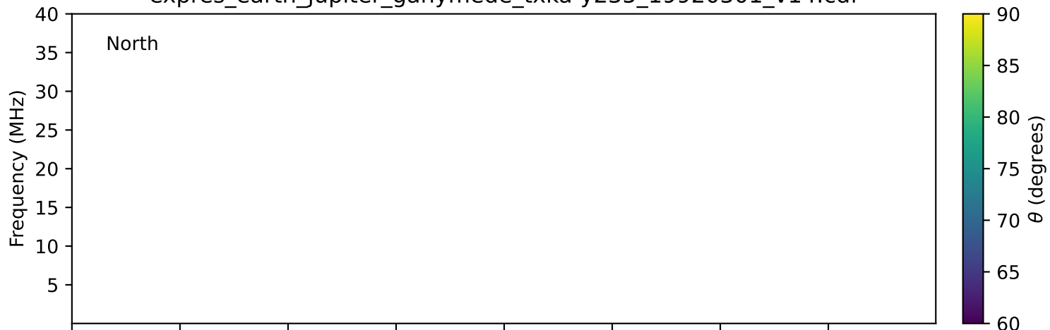
expres_earth_jupiter_ganymede_txka-y235_19920301_v14.cdf
