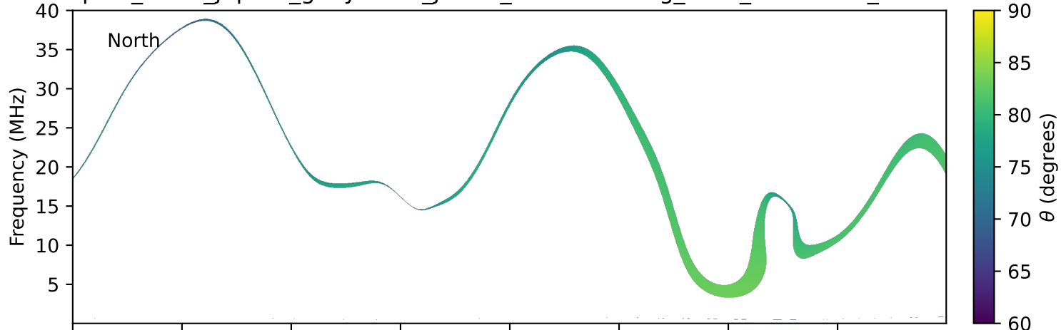
expres_earth_jupiter_ganymede_jrm33_lossc-wid1deg_3kev_19920326_v11.cdf
