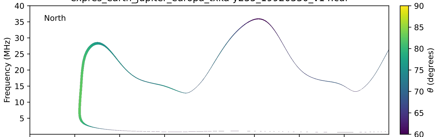
expres_earth_jupiter_europa_txka-y235_19920330_v14.cdf
