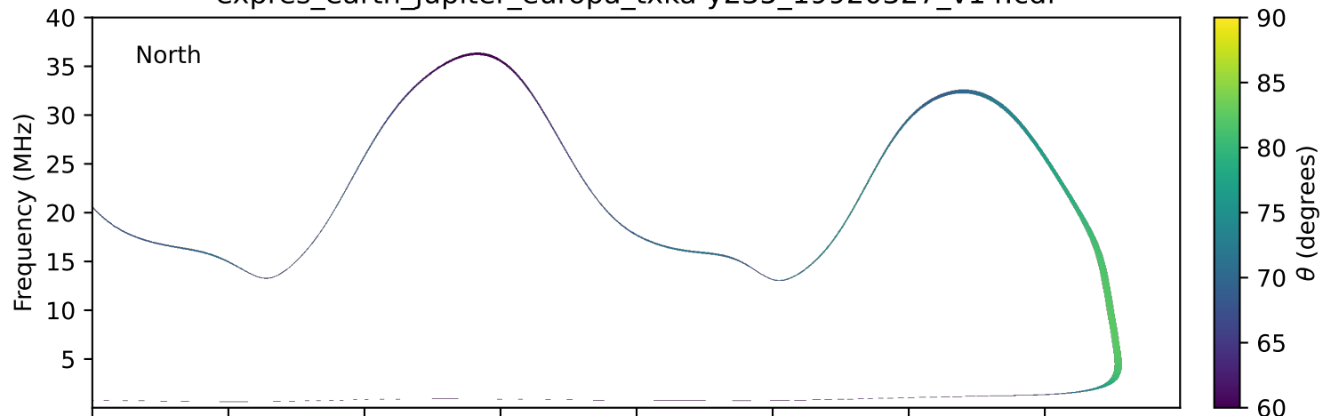
expres_earth_jupiter_europa_txka-y235_19920327_v14.cdf
