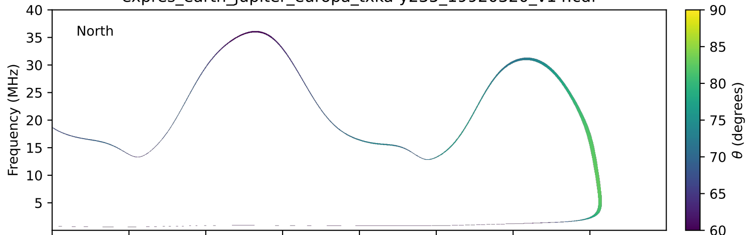
expres_earth_jupiter_europa_txka-y235_19920320_v14.cdf
