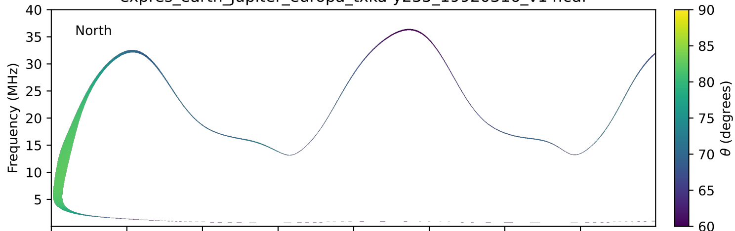
expres_earth_jupiter_europa_txka-y235_19920316_v14.cdf
