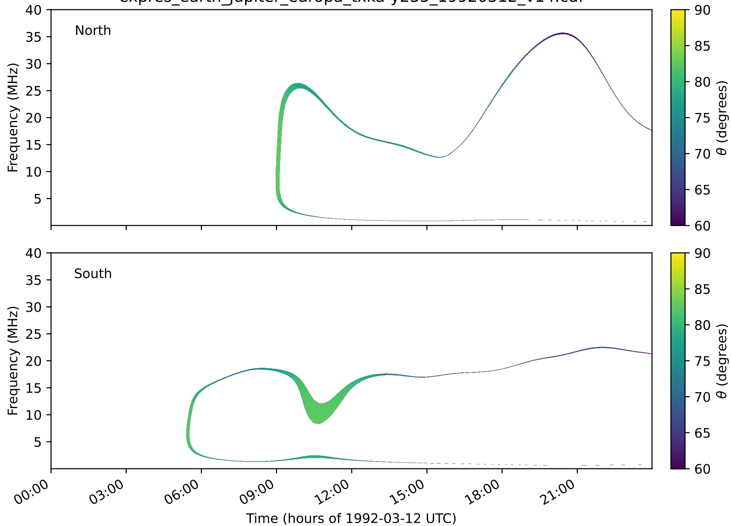
expres_earth_jupiter_europa_txka-y235_19920312_v14.cdf
