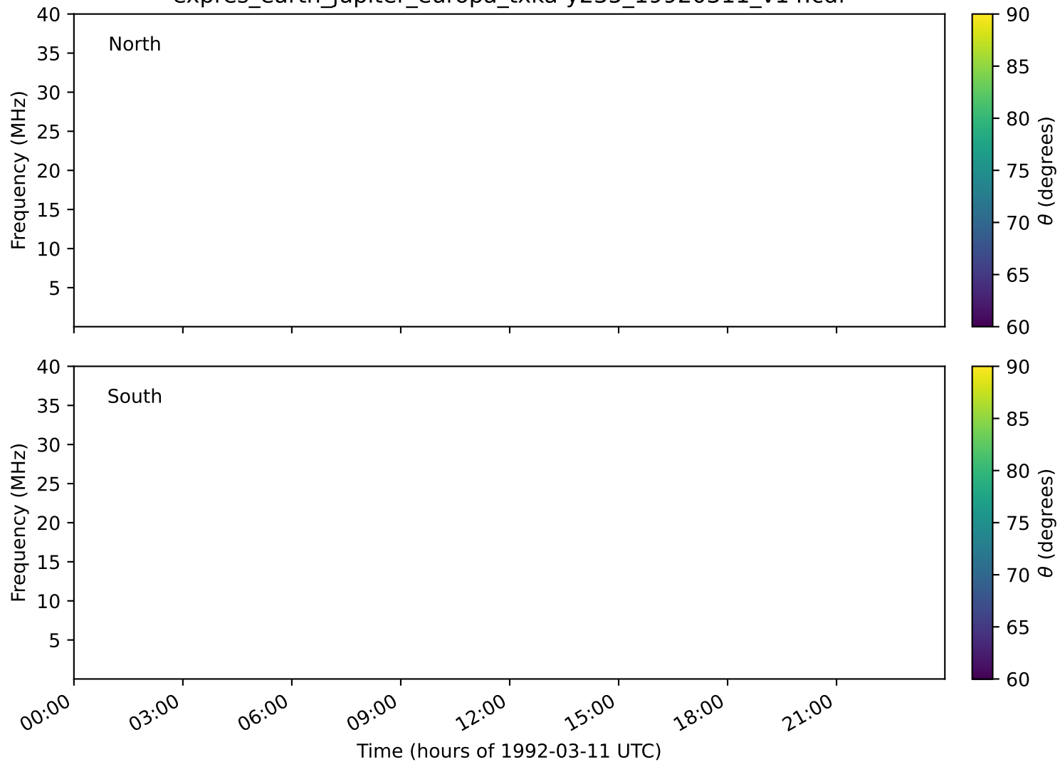
expres_earth_jupiter_europa_txka-y235_19920311_v14.cdf
