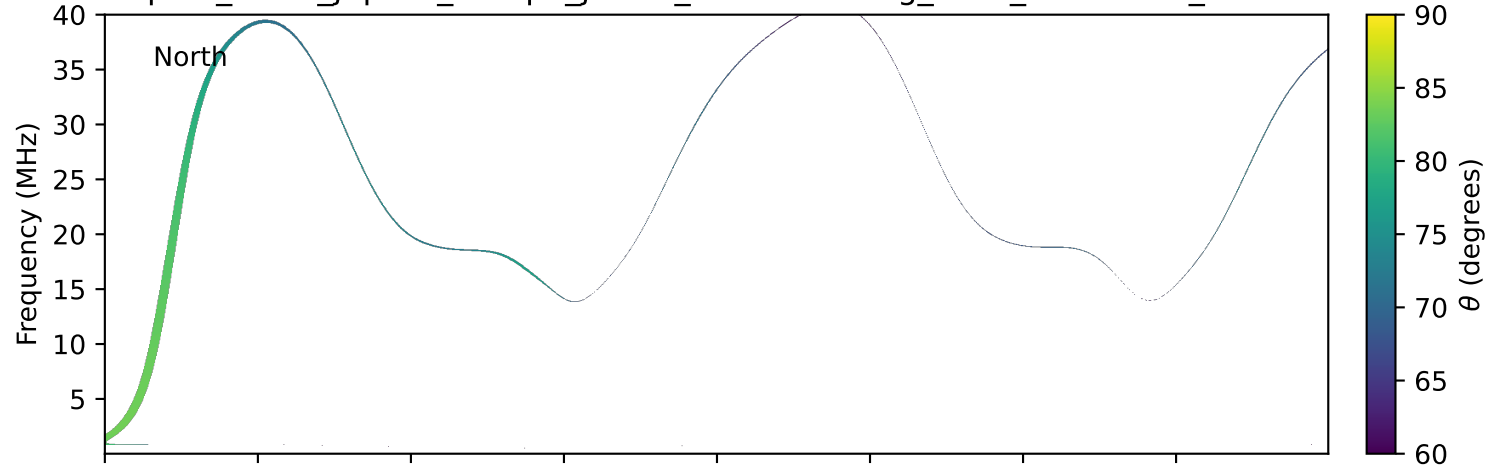
expres_earth_jupiter_europa_jrm33_lossc-wid1deg_3kev_19920316_v11.cdf
