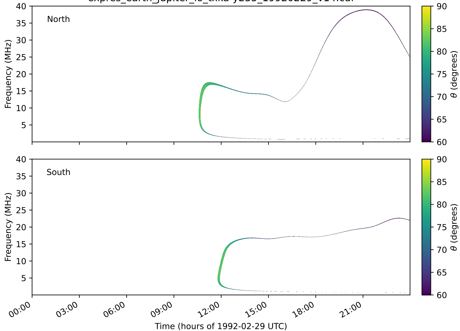
expres_earth_jupiter_io_txka-y235_19920229_v14.cdf
