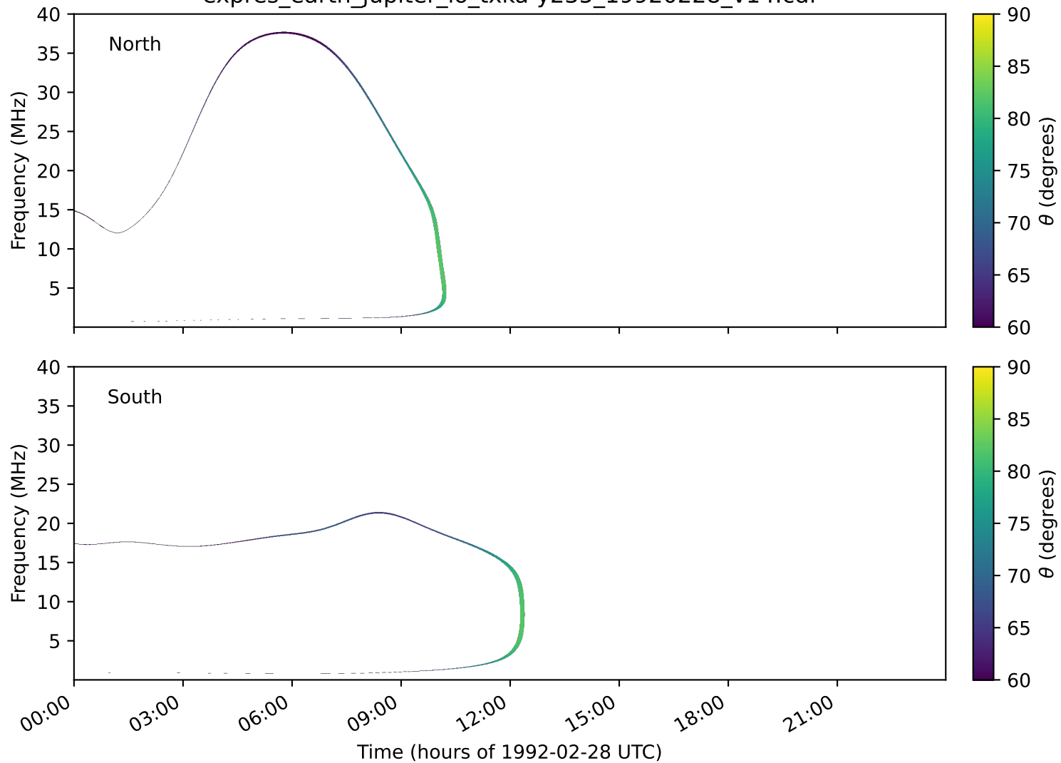
expres_earth_jupiter_io_txka-y235_19920228_v14.cdf
