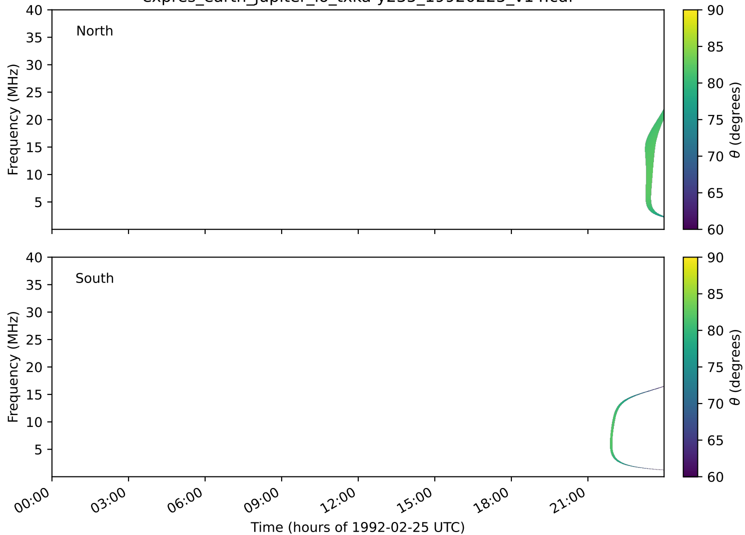
expres_earth_jupiter_io_txka-y235_19920225_v14.cdf
