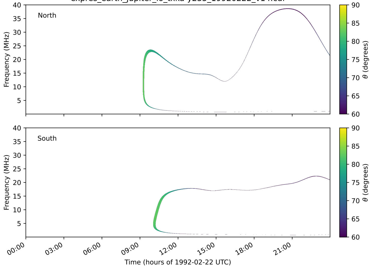
expres_earth_jupiter_io_txka-y235_19920222_v14.cdf
