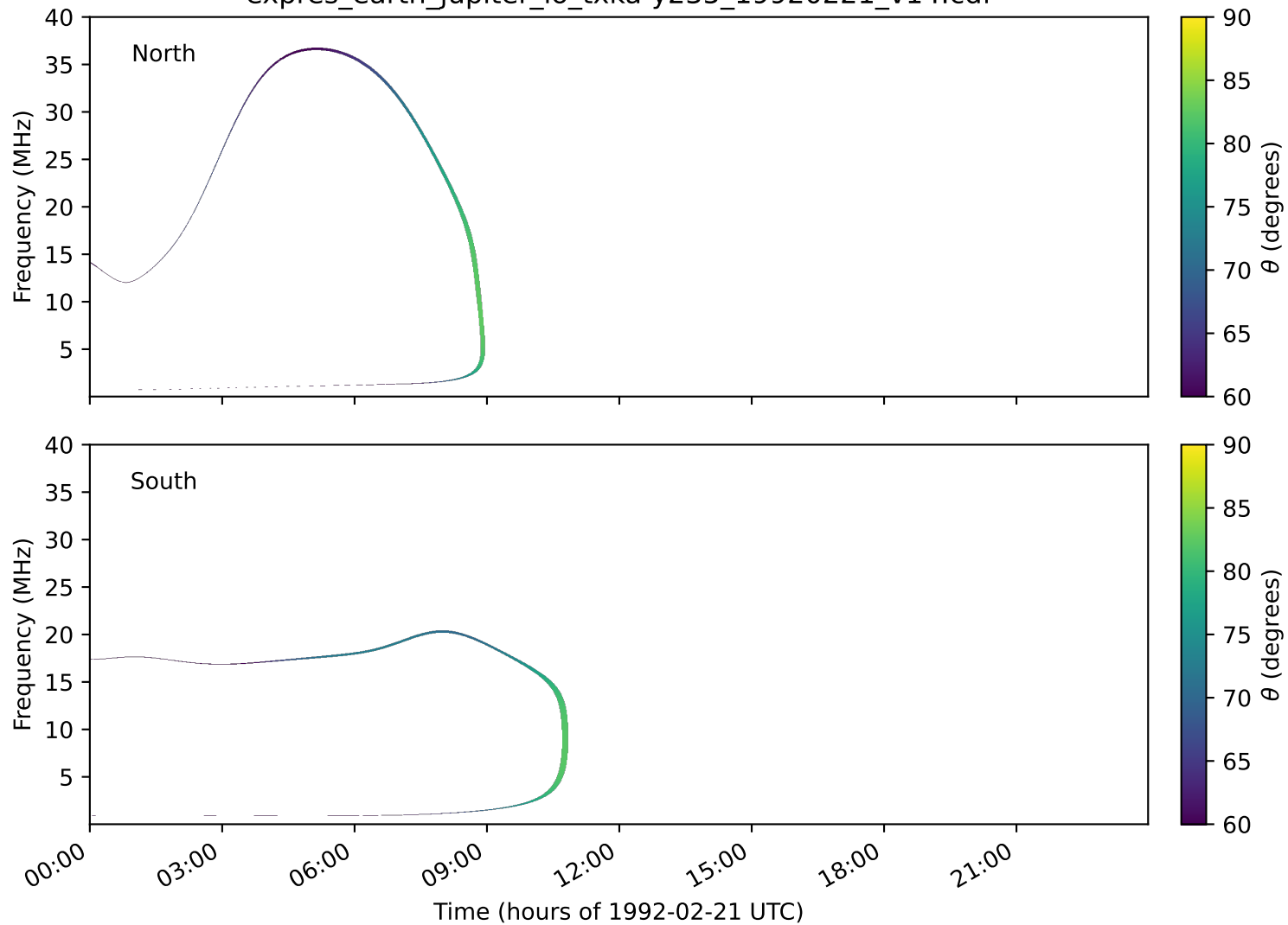
expres_earth_jupiter_io_txka-y235_19920221_v14.cdf
