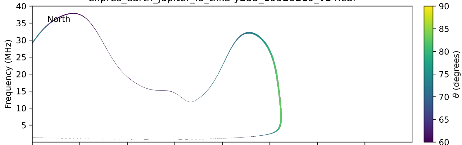
expres_earth_jupiter_io_txka-y235_19920219_v14.cdf
