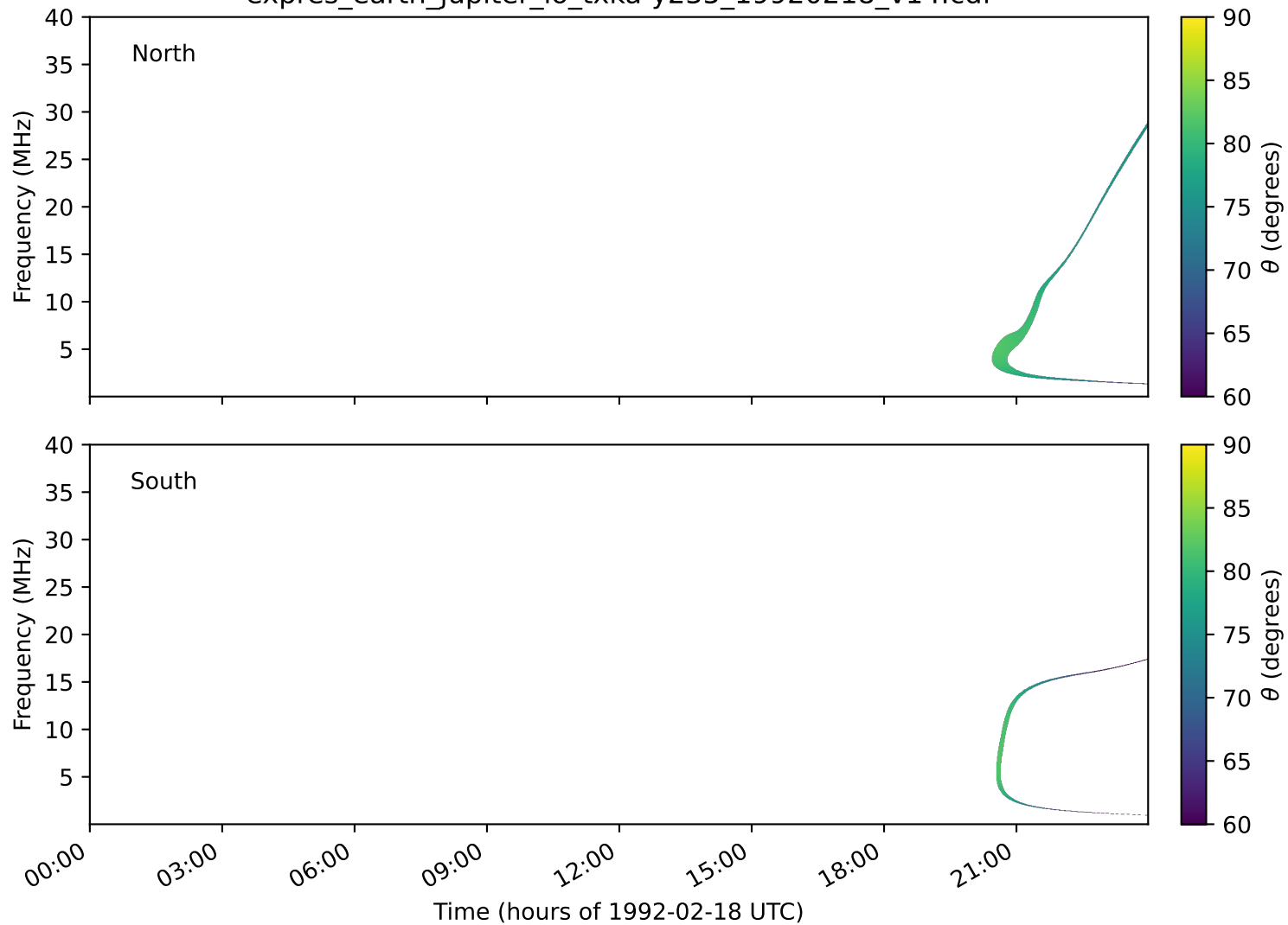
expres_earth_jupiter_io_txka-y235_19920218_v14.cdf
