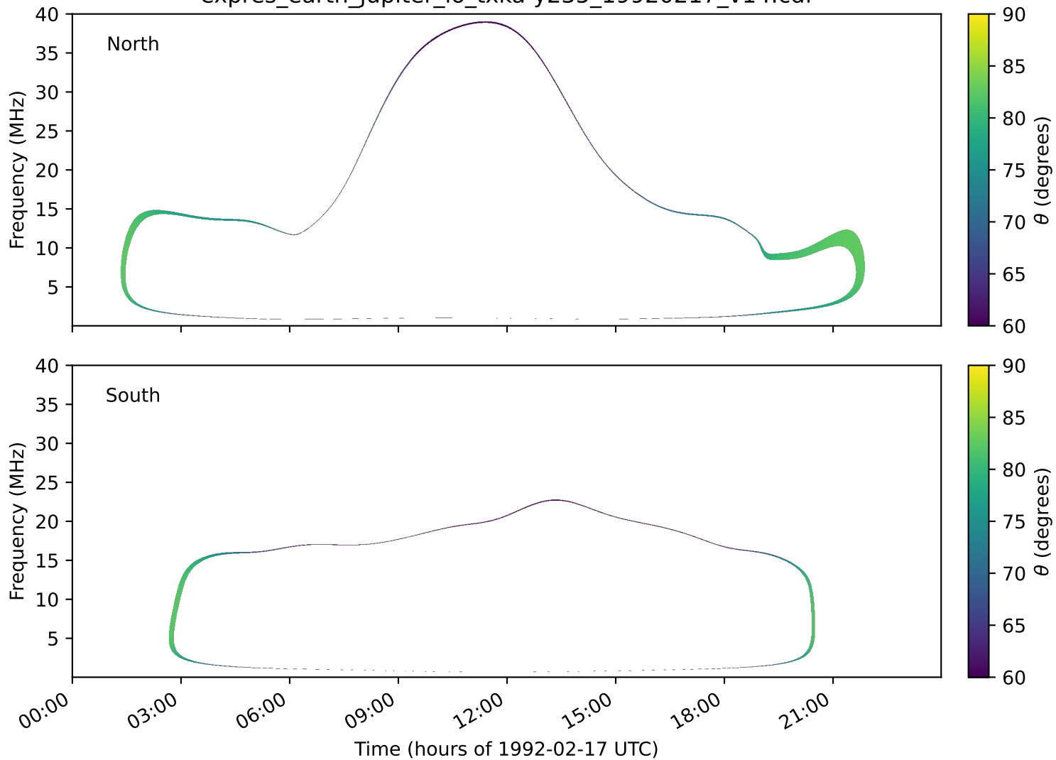
expres_earth_jupiter_io_txka-y235_19920217_v14.cdf
