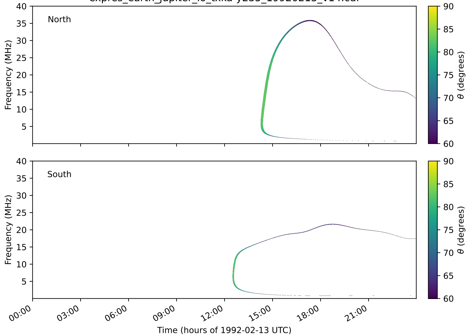
expres_earth_jupiter_io_txka-y235_19920213_v14.cdf
