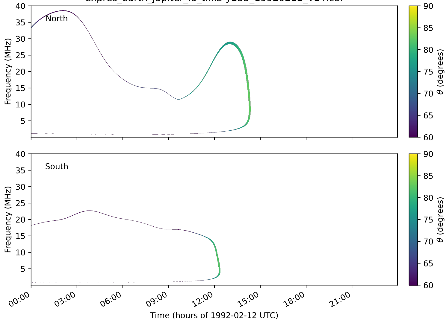
expres_earth_jupiter_io_txka-y235_19920212_v14.cdf
