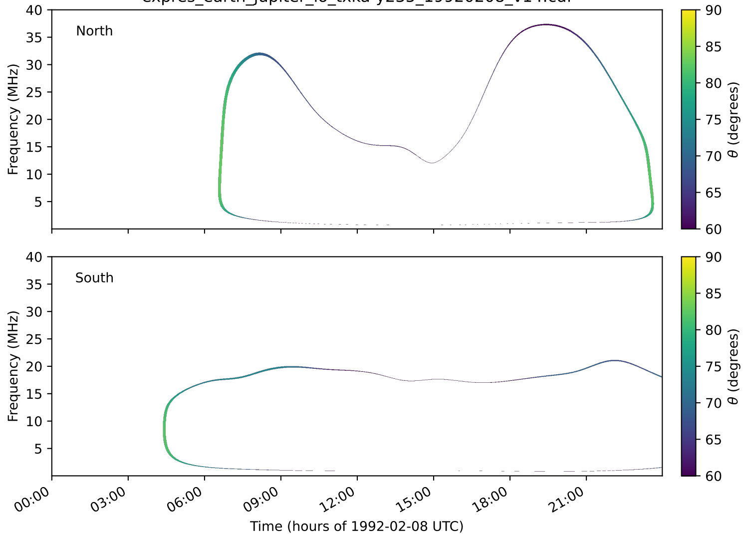
expres_earth_jupiter_io_txka-y235_19920208_v14.cdf
