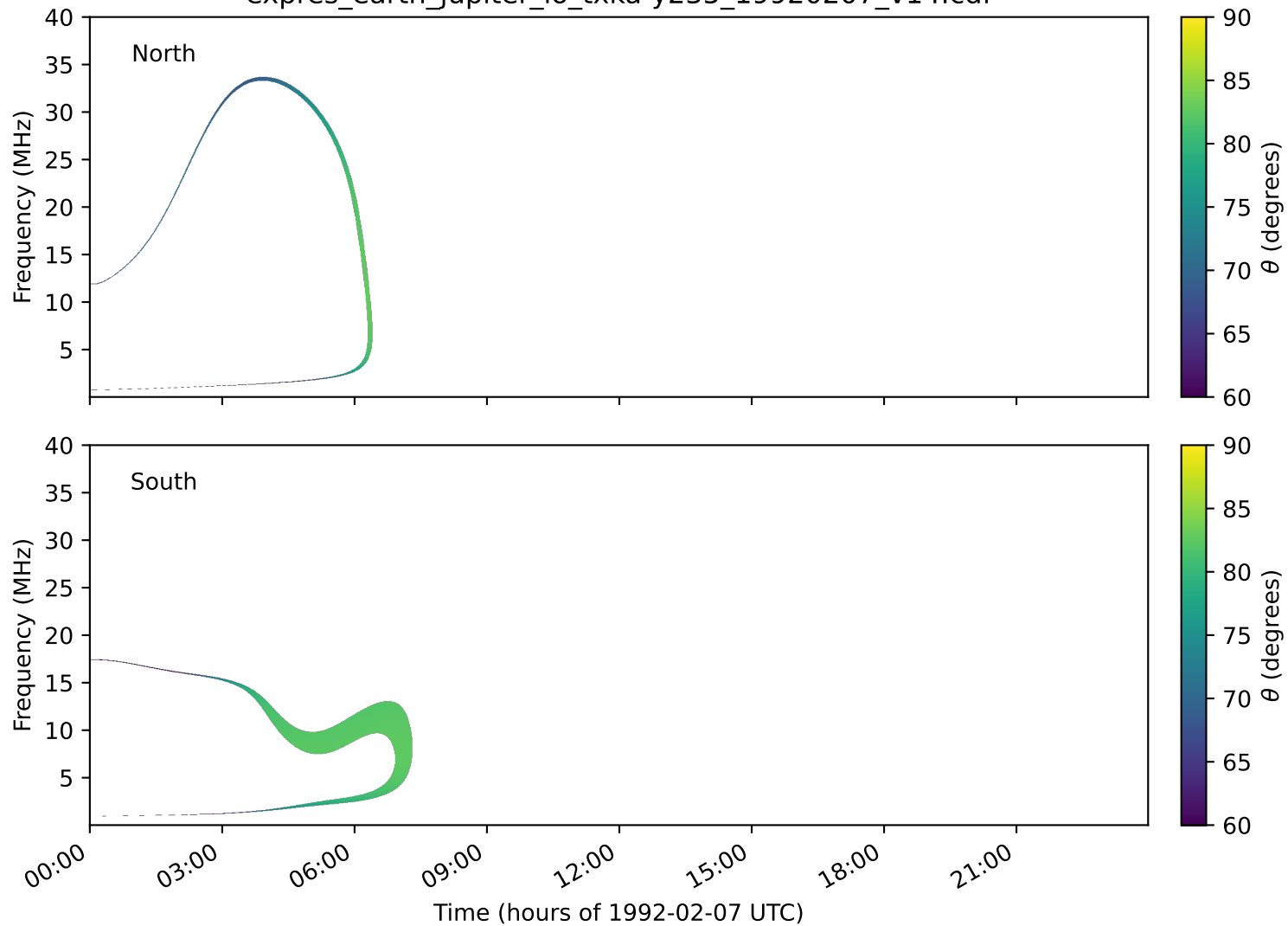
expres_earth_jupiter_io_txka-y235_19920207_v14.cdf
