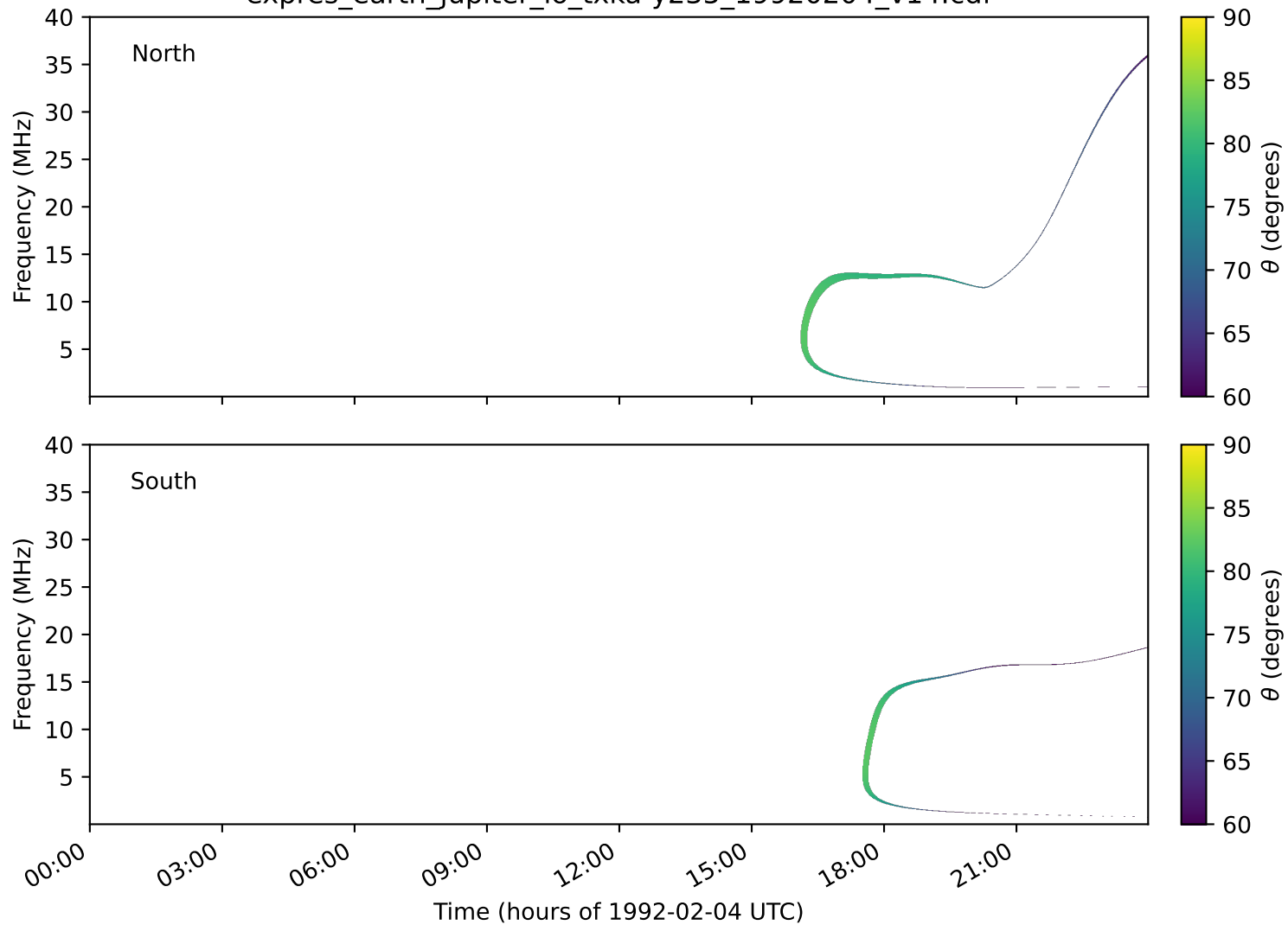
expres_earth_jupiter_io_txka-y235_19920204_v14.cdf
