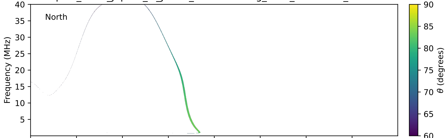
expres_earth_jupiter_io_jrm33_lossc-wid1deg_3kev_19920228_v11.cdf
