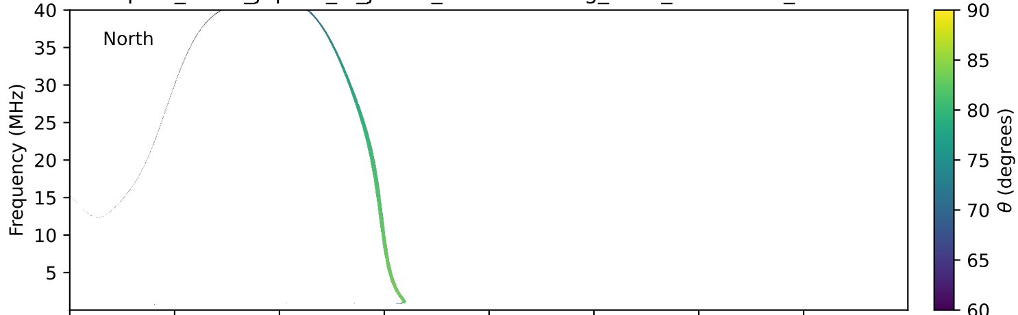
expres_earth_jupiter_io_jrm33_lossc-wid1deg_3kev_19920221_v11.cdf
