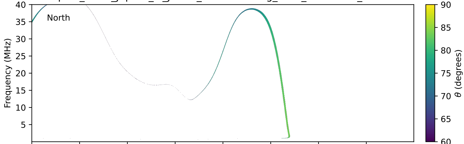
expres_earth_jupiter_io_jrm33_lossc-wid1deg_3kev_19920219_v11.cdf
