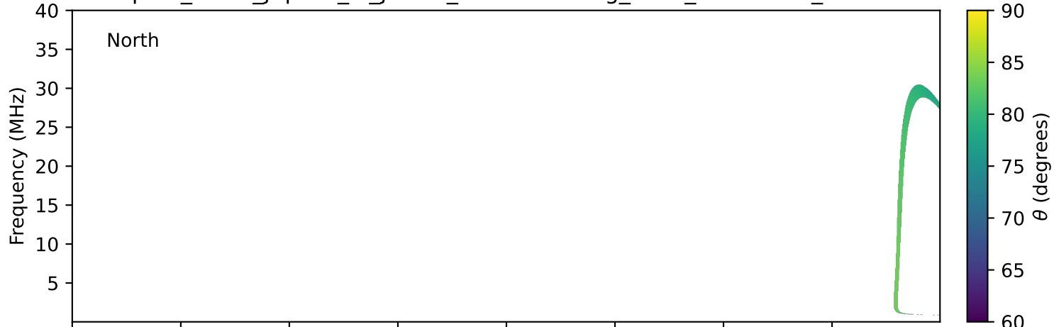
expres_earth_jupiter_io_jrm33_lossc-wid1deg_3kev_19920202_v11.cdf
