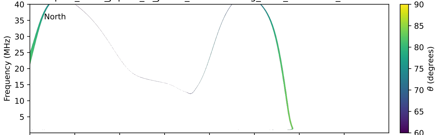
expres_earth_jupiter_io_jrm09_lossc-wid1deg_3kev_19920226_v11.cdf
