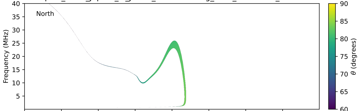
expres_earth_jupiter_io_jrm09_lossc-wid1deg_3kev_19920205_v11.cdf
