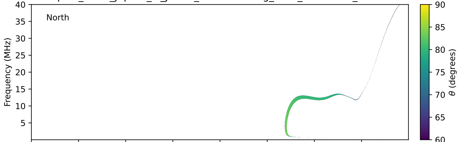
expres_earth_jupiter_io_jrm09_lossc-wid1deg_3kev_19920204_v11.cdf
