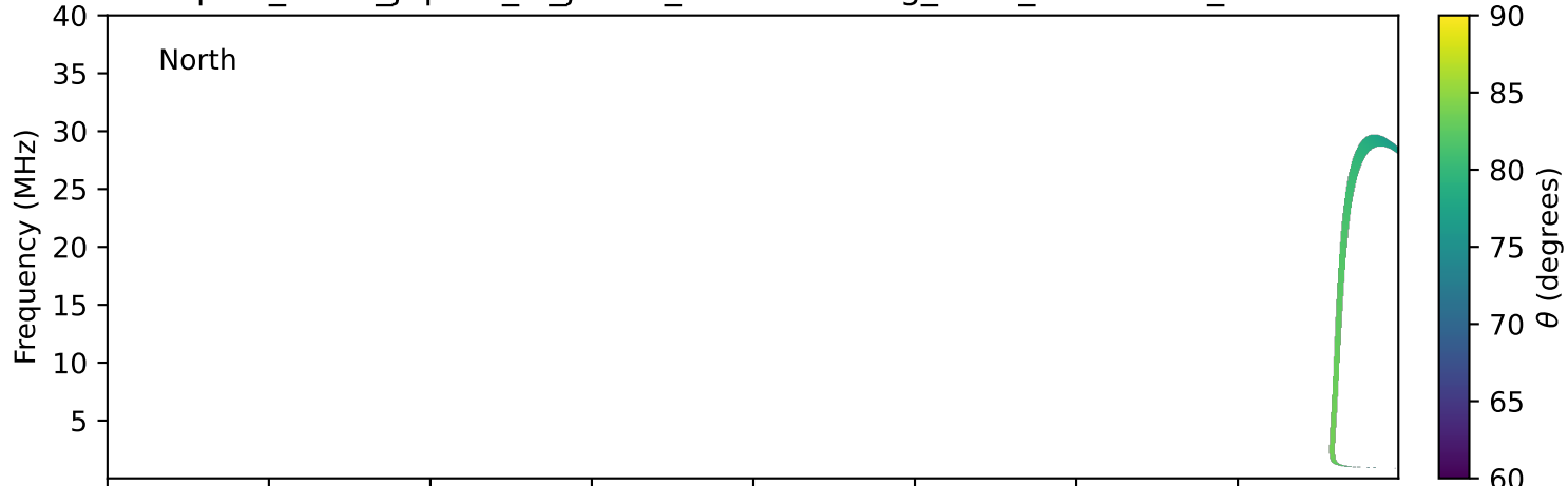
expres_earth_jupiter_io_jrm09_lossc-wid1deg_3kev_19920202_v11.cdf
